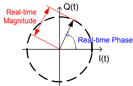
Figure 9. Cordic Extraction
