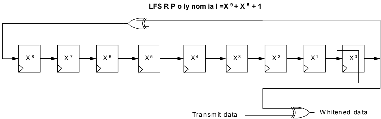
Figure 37. Data Whitening
