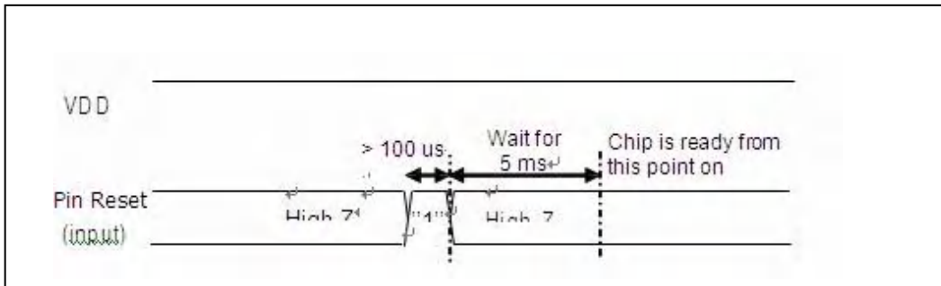
Figure 39. Manual Reset Timing Diagram
