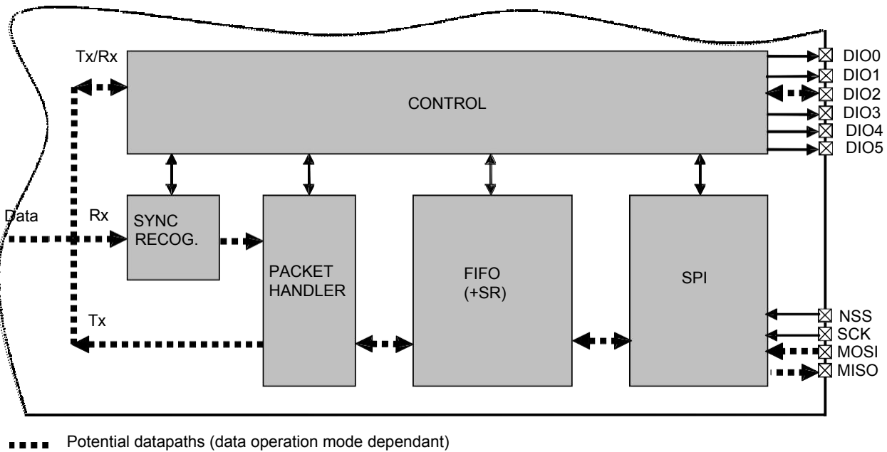
Figure 23. DL-RFM69HC Data Processing Conceptual View
