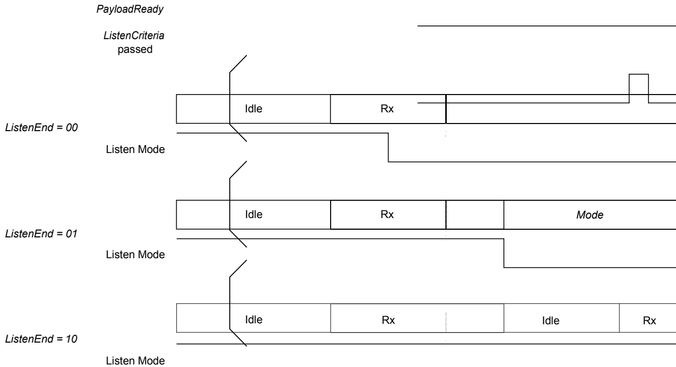
Figure 21. Listen Mode Sequence (wanted signal is received)
